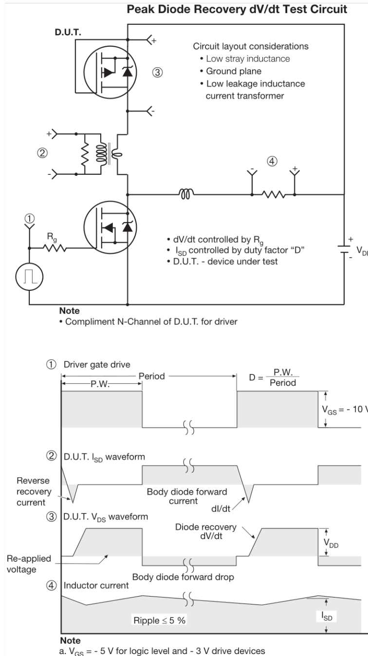
Fig. 14 - For P-Channel
