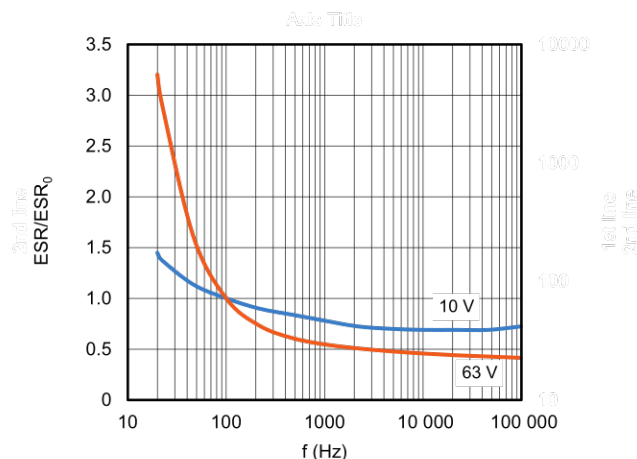
Fig. 8 - Typical multiplier of ESR as a function of frequency ( ESR_0 = typical ESR at 100 Hz at 20 °C)
