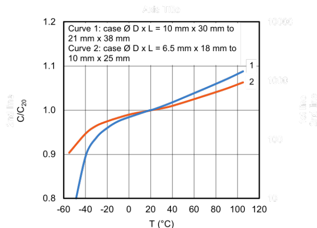
Fig. 5 - Typical multiplier of capacitance as a function of ambient temperature ( C_{20} = capacitance at 20 °C, 100 Hz)
