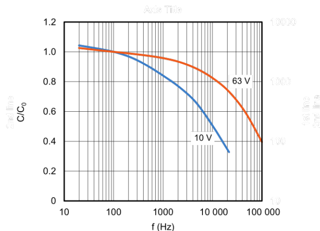
Fig. 6 - Typical multiplier of capacitance as a function of frequency ( C_0 = typical capacitance at 100 Hz at 20 °C)
