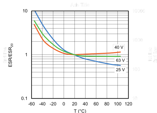
Fig. 7 - Typical multiplier of ESR as a function of ambient temperature ( ESR_{20} = typical ESR at 100 Hz at 20 °C)
