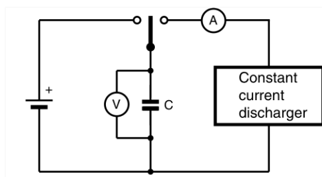
Fig.5 Test circuit for capacitance measurement
