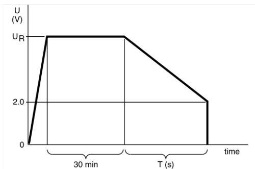
Fig.4 Voltage diagram for capacitance measurement
