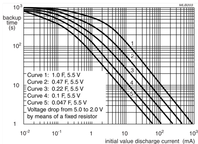
Fig.11 Typical backup time as a function of initial discharge current
