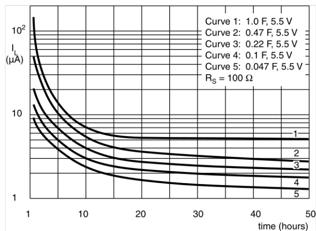
Fig.8 Typical leakage current as a function of time
