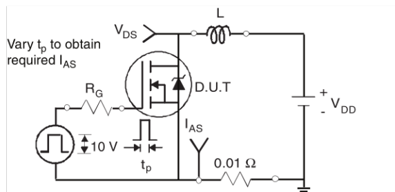
Fig. 12a - Unclamped Inductive Test Circuit
