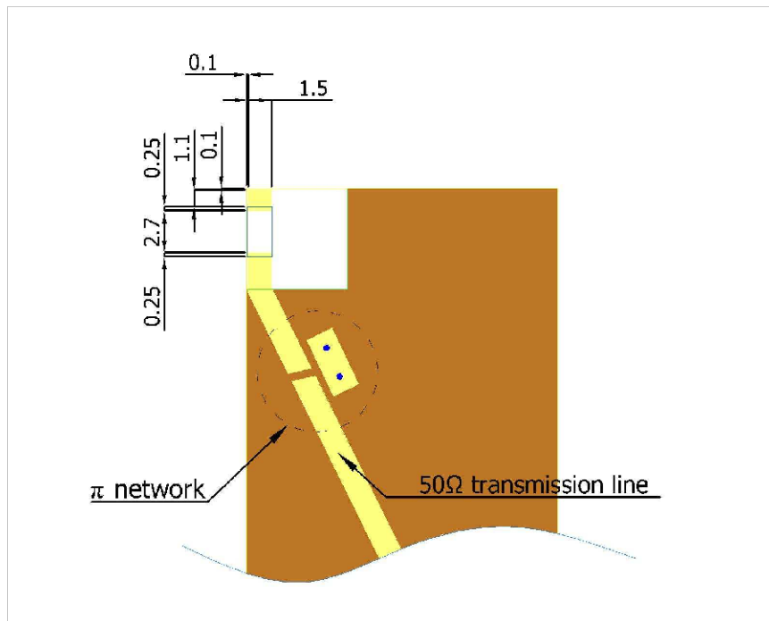
Land Pattern
