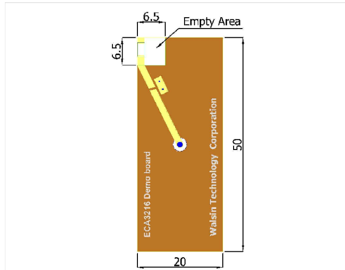
Land Pattern
