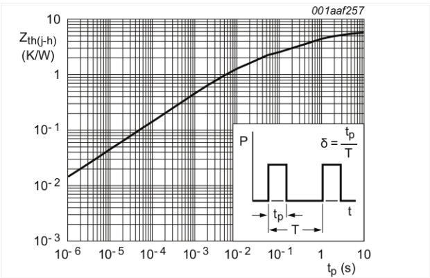
Fig. 4. Transient thermal impedance from junction to heatsink as a function of pulse duration
