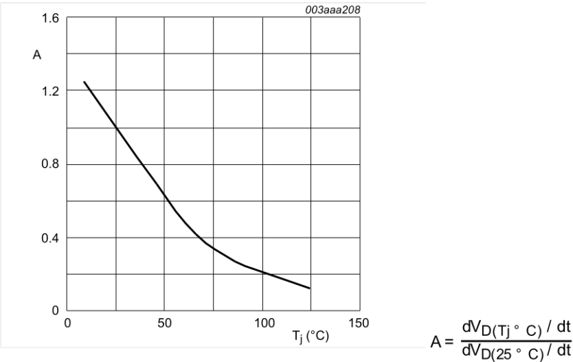
Fig. 13. Normalized critical rate of rise of off-state voltage as a function of junction temperature; typical values
