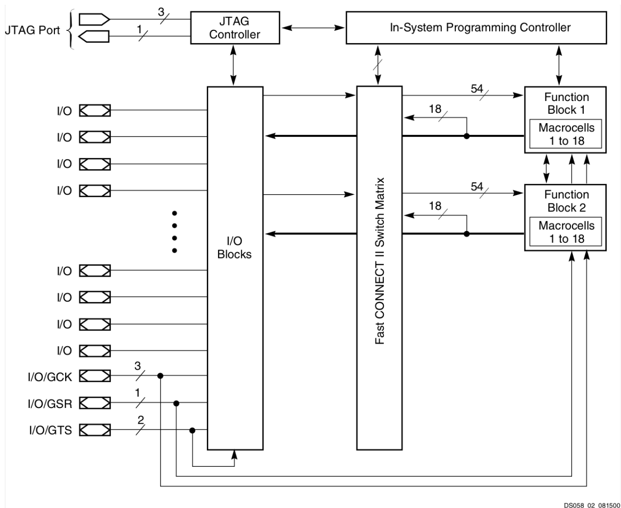
Figure 2: XC9536XL Architecture
