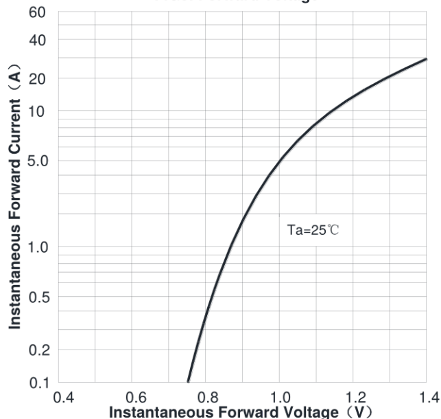
FIG3: Forward Voltage
